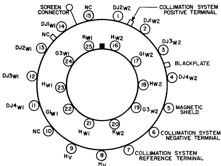
TERMINAL DIAGRAM (Bottom View)
